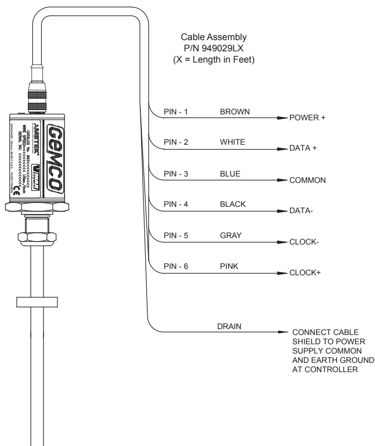
Figure 3-1: Wiring for Connector Option "S", 6 Pin 12 mm Micro
