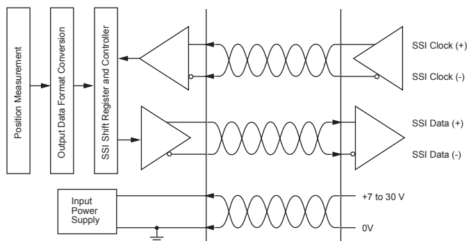
SSI Logic Diagram
