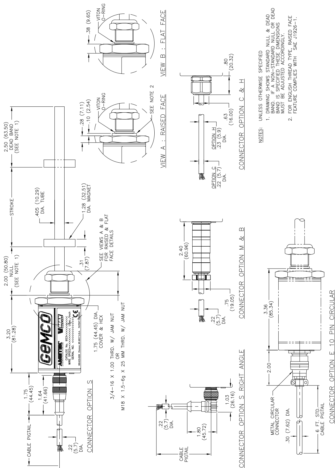
Figure 1-1 953SSI Dimension Drawing
